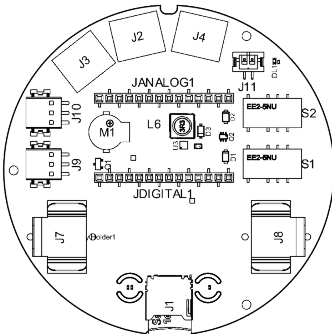
Bottom view
