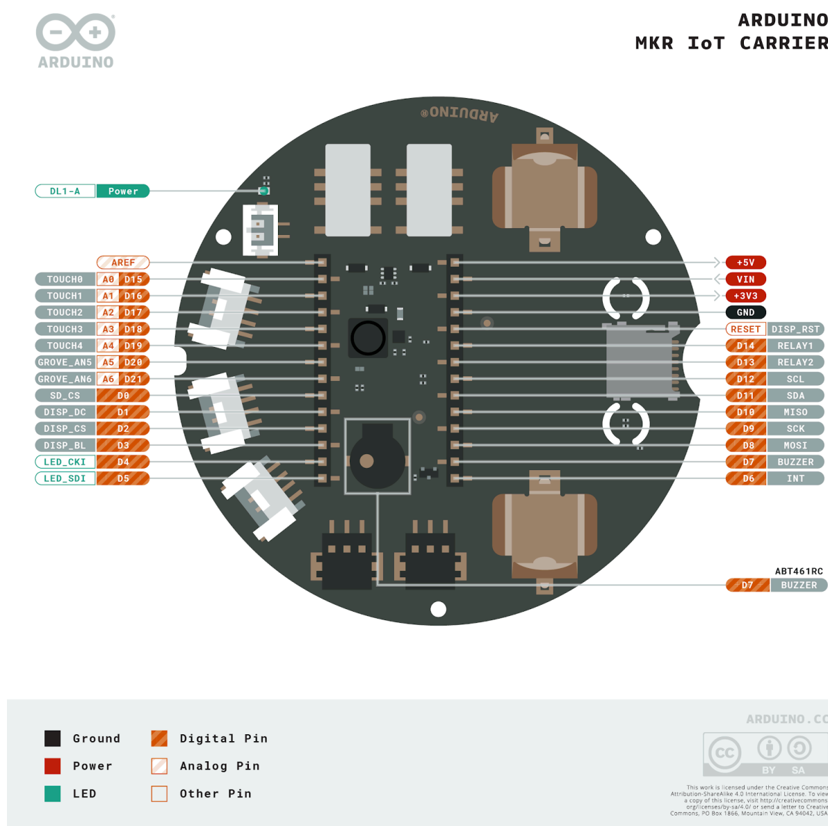
Pinout
